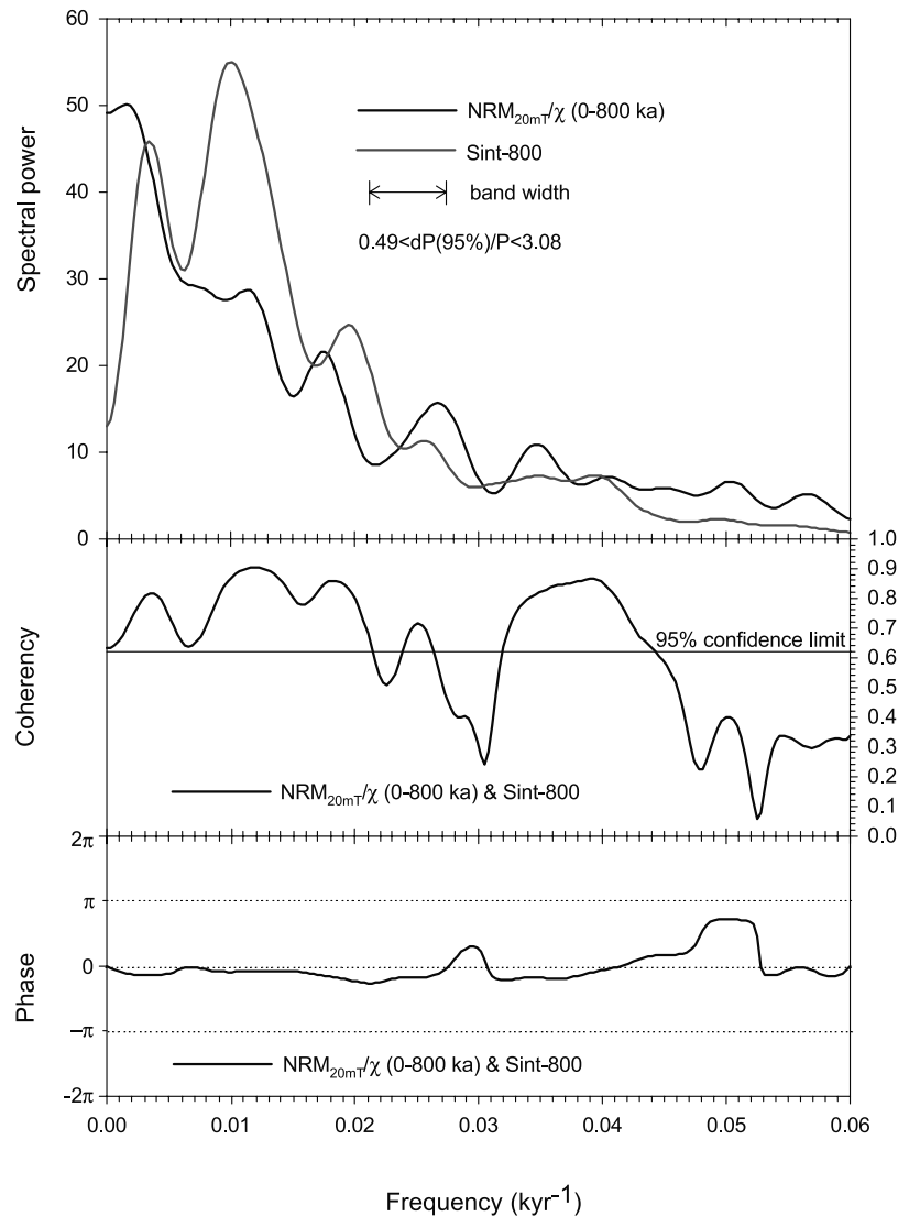
Figure 9. Spectral power, coherency and phase resulting from cross-spectral analysis of \text{NRM}_{20\text{mT}}/\chi for core MD972143 and the Sint-800 paleointensity stack of Guyodo and Valet [1999] for the last 800 kyr. There is significant coherency between both signals across a broad range of frequencies, which suggests that the records are quantitatively similar.
