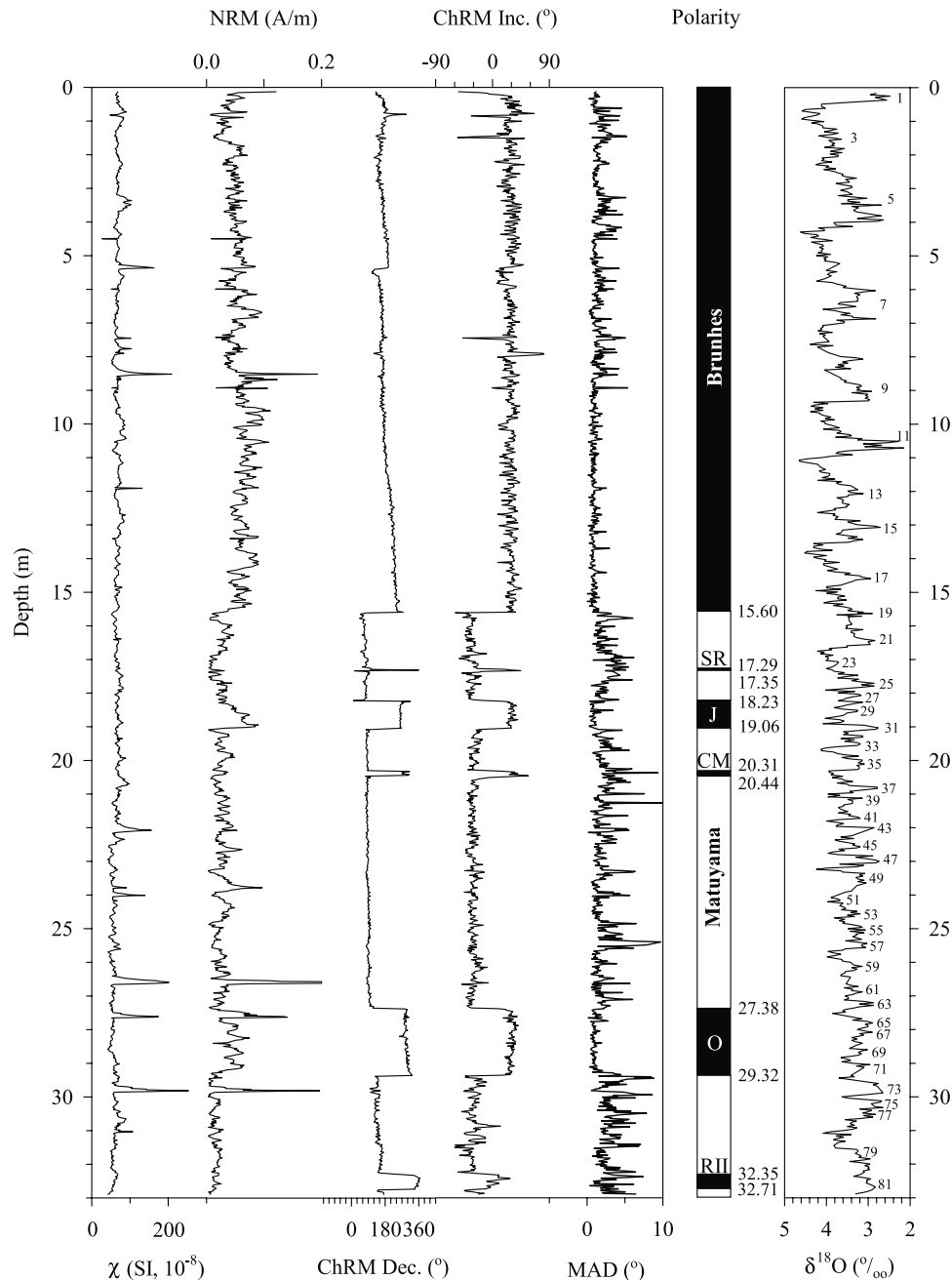
Figure 2. Magnetic properties and chronostratigraphic framework for core MD972143. From left to right, versus depth: low-field magnetic susceptibility ( \chi ), intensity of the natural remanent magnetization (NRM) prior to demagnetization, declination and inclination, respectively, of the characteristic remanent magnetization (ChRM), which was calculated using data from multiple demagnetization steps, maximum angular deviation (MAD) values associated with the ChRM determinations, polarity (black, normal; white, reversed), with depths indicated for polarity boundaries (SR, Santa Rosa polarity interval; J, Jaramillo Subchron; CM, Cobb Mountain Subchron; O, Olduvai Subchron; and RII, Réunion II Subchron), and \delta^{18}\text{O} variations, with numbers indicating \delta^{18}\text{O} stages after Shackleton and Pisias [1985], Shackleton et al. [1990], and Shackleton et al. [1995]. Peaks in magnetic susceptibility and NRM represent volcanic ash layers.
