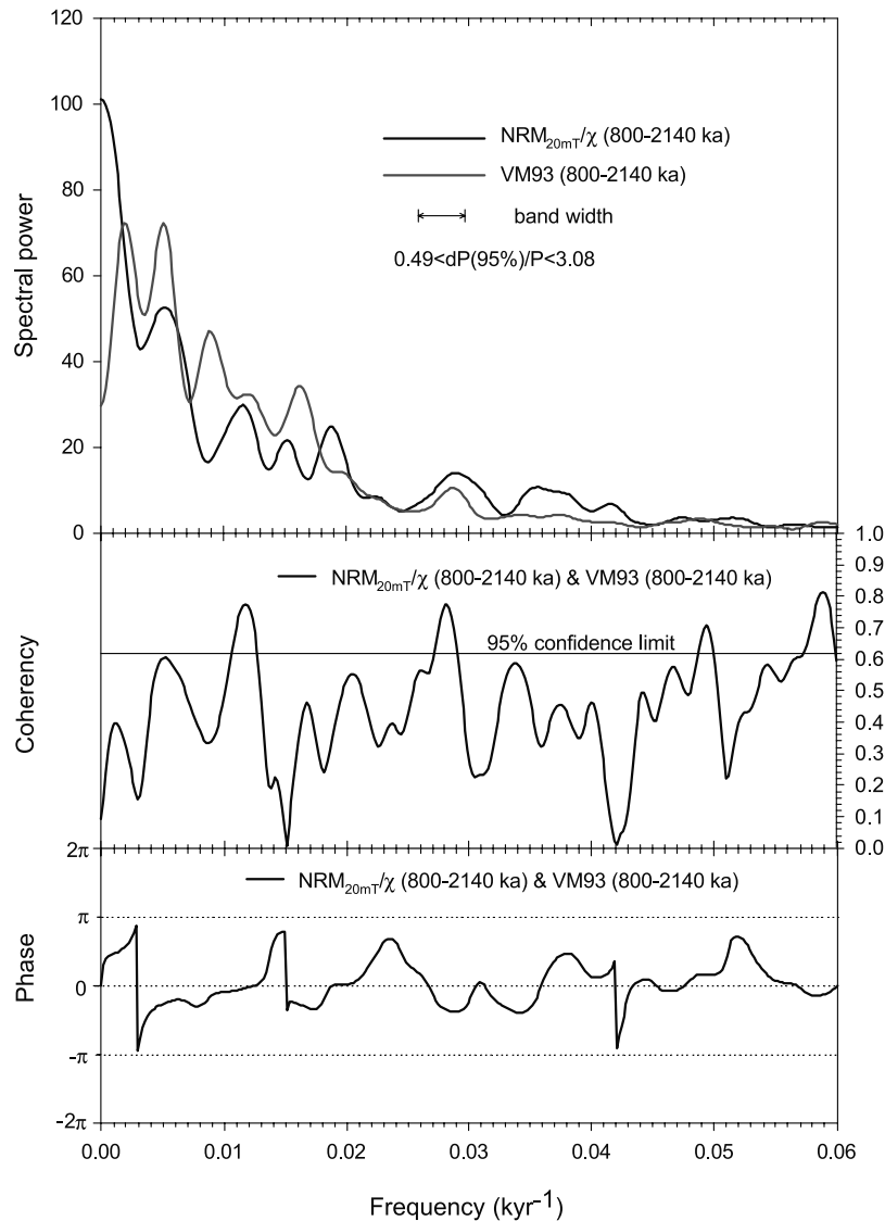
Figure 10. Spectral power, coherency and phase resulting from cross-spectral analysis of \text{NRM}_{20\text{mT}}/\chi for core MD972143 and the equatorial Pacific paleointensity record of Valet and Meynadier [1993] (VM93) for the interval from 800 ka to 2.14 Ma. Coherency between these records is poor compared to that between core MD972143 and the Sint-800 paleointensity stack, as shown in Figure 9 (see text for discussion).
