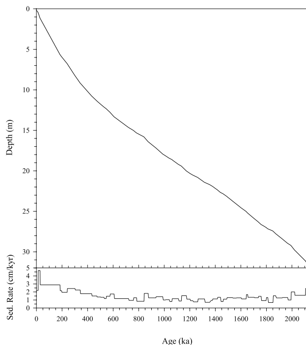
Figure 3. Depth versus age plot for core MD972143, using the astronomically tuned age model of Hornig et al. [2002], which was constructed after subtraction of 0.93 m of sediment represented by volcanic ash layers. Variations in sedimentation rate throughout the studied age interval are shown in the bottom panel.
