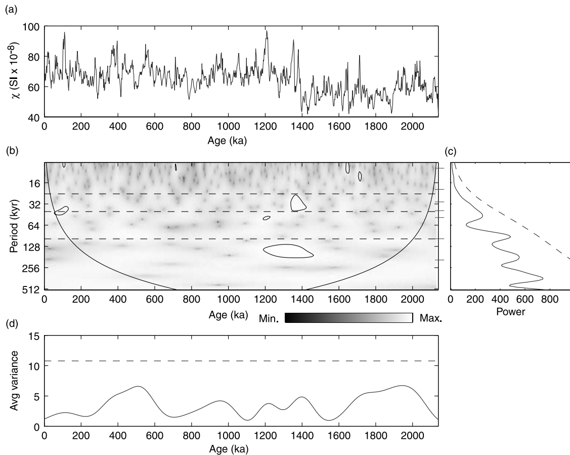
Figure 7. Wavelet analysis of the relative paleointensity normalizing parameter ( \chi ) for core MD972143. (a) Magnetic susceptibility ( \chi ) for the studied 2.14 Myr time series. (b) Wavelet power spectrum for the \chi time series (compare Figure 6). (c) Global wavelet spectrum for the entire \chi time series. The dashed line indicates the 95% confidence interval (i.e., none of the spectral peaks are globally significant). (d) The scale-averaged variance of the wavelet power spectrum, which shows the localization of spectral power for periods ranging from 90 to 110 kyr.
