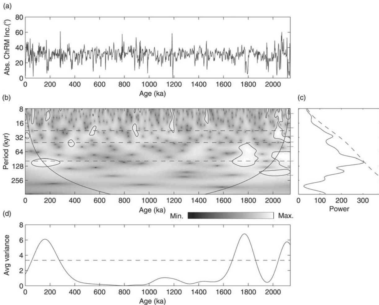
Figure 12. Wavelet analysis of the absolute value of the paleomagnetic inclinations for core MD972143. (a) Absolute value of the paleomagnetic inclination for the studied 2.14 Myr time series. (b) Wavelet power spectrum for the inclination time series (compare. Figure 6). (c) Global wavelet spectrum for the entire inclination time series. The dashed line indicates the 95% confidence level. (d) The scale averaged variance of the wavelet power spectrum, which shows the localization of spectral power for periods ranging from 90 to 110 kyr.
