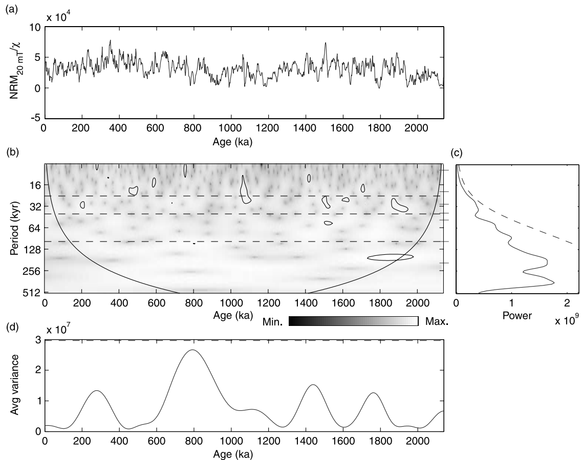
Figure 6. Wavelet analysis of the relative paleointensity proxy ( \text{NRM}_{20\text{mT}}/\chi ) for core MD972143. (a) \text{NRM}_{20\text{mT}}/\chi for the studied 2.14 Myr time series. (b) Wavelet power spectrum for the paleointensity time series. Orbital periods of precession (23 kyr), obliquity (41 kyr), and eccentricity (100 kyr) are shown as dashed lines. Other ticks on the right-hand scale indicate periods of 10, 20, 30, 40, 50, and 200 kyr. Contour lines surrounding intervals with light shading indicate statistically significant power at the 95% confidence level for red noise with a lag 1 autoregressive process [see Torrence and Campo , 1998]. Curved lines on either side of the figure indicate the “cone of confidence” where edge effects become important. (c) Global wavelet spectrum for the entire paleointensity time series. The dashed line indicates the 95% confidence level (i.e., none of the spectral peaks are globally significant). (d) The scale-averaged variance of the wavelet power spectrum, which shows the localization of spectral power for periods ranging from 90 to 110 kyr.
