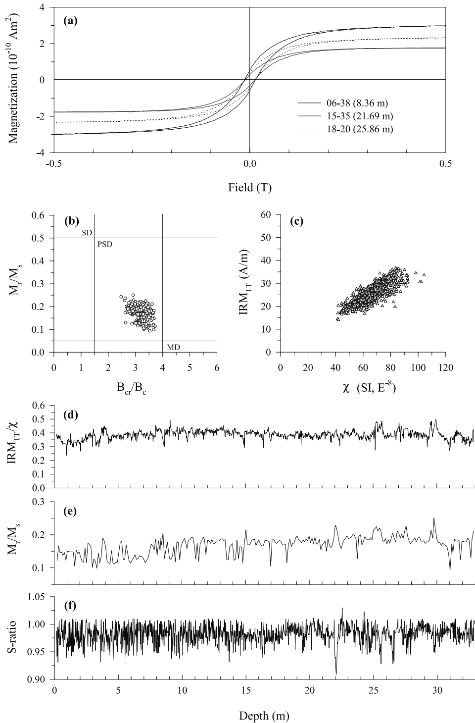
Figure 4. Mineral magnetic properties for core MD972143. (a) Representative hysteresis loops. (b) Plot of M_r/M_s versus B_{cr}/B_c for 313 samples [Day et al. , 1977], which indicates that the magnetic mineral assemblage is dominated by pseudosingle-domain (PSD) titanomagnetite (SD, single domain, and MD, multidomain). (c) Plot of IRM_{1T} versus \chi for all samples except those from volcanic ash horizons which are not considered for paleointensity determinations. The clustering of the data indicates that the titanomagnetite particles have a relatively narrow range of concentrations and the near linearity of the cluster indicates that the range of grain size variation is also narrow. If a line of best fit is fitted through the data, it would have a positive intercept on the horizontal axis, which indicates that paramagnetic minerals contribute to the susceptibility. (d) and (e) Down-core variations of grain-size-dependent magnetic parameters IRM_{1T}/\chi and M_r/M_s , respectively. (f) Down-core variations of the S ratio indicate that a ferrimagnetic mineral dominates the magnetic properties. This is consistent with the identification of titanomagnetite [Horng et al. , 2002].
