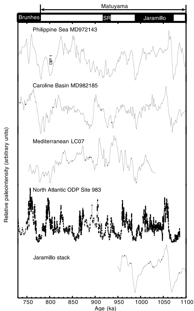
Figure 11. Comparison of paleointensity records between 0.73 and 1.10 Ma, including the records from core MD972143, West Caroline Basin core MD982185 [Yamazaki and Oda, 2002], Mediterranean core LC07 [Dinarès-Turell et al., 2002], North Atlantic ODP Site 983 [Channell and Kleiven, 2000], and the Jaramillo paleointensity stack of Guyodo et al. [2001].
