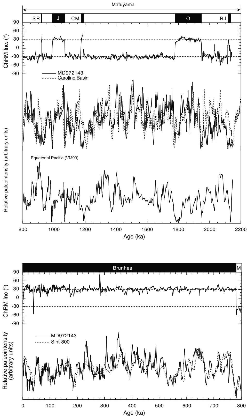
Figure 8. The relative paleointensity record for core MD972143 compared to the Sint-800 global paleointensity stack [Guyodo and Valet, 1999] for the last 800 kyr and compared to the West Caroline Basin record of Yamazaki and Oda [2002] and the equatorial Pacific paleointensity record of Valet and Meynadier [1993] (VM93) for the interval from 800 ka to 2.14 Ma. ChRM inclinations are also shown to indicate the positions of polarity reversals documented in core MD972143 (dotted lines indicate the inclinations expected for a geocentric axial dipole field at the site latitude). Black, normal polarity, and white, reversed polarity on the polarity log, which has the same labels as in Figure 2.
