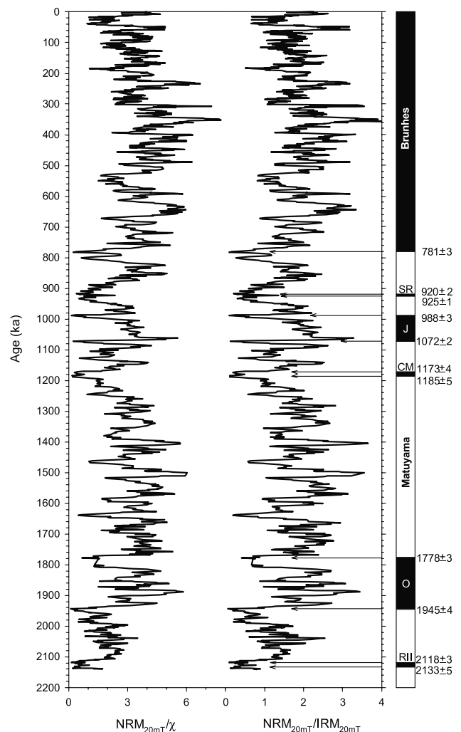
Figure 5. Two estimates of relative geomagnetic paleointensity for the last 2.14 Myr from core MD972143: \text{NRM}_{20\text{mT}}/\chi and \text{NRM}_{20\text{mT}}/\text{IRM}_{20\text{mT}} . Ages are plotted with respect to the astronomically tuned age model of Hornig et al. [2002]. The magnetic polarity zonation for the core is summarized on the right-hand side of the figure, along with the ages derived for the polarity boundaries by Hornig et al. [2002]. Abbreviations for polarity intervals are the same as in Figure 2.
